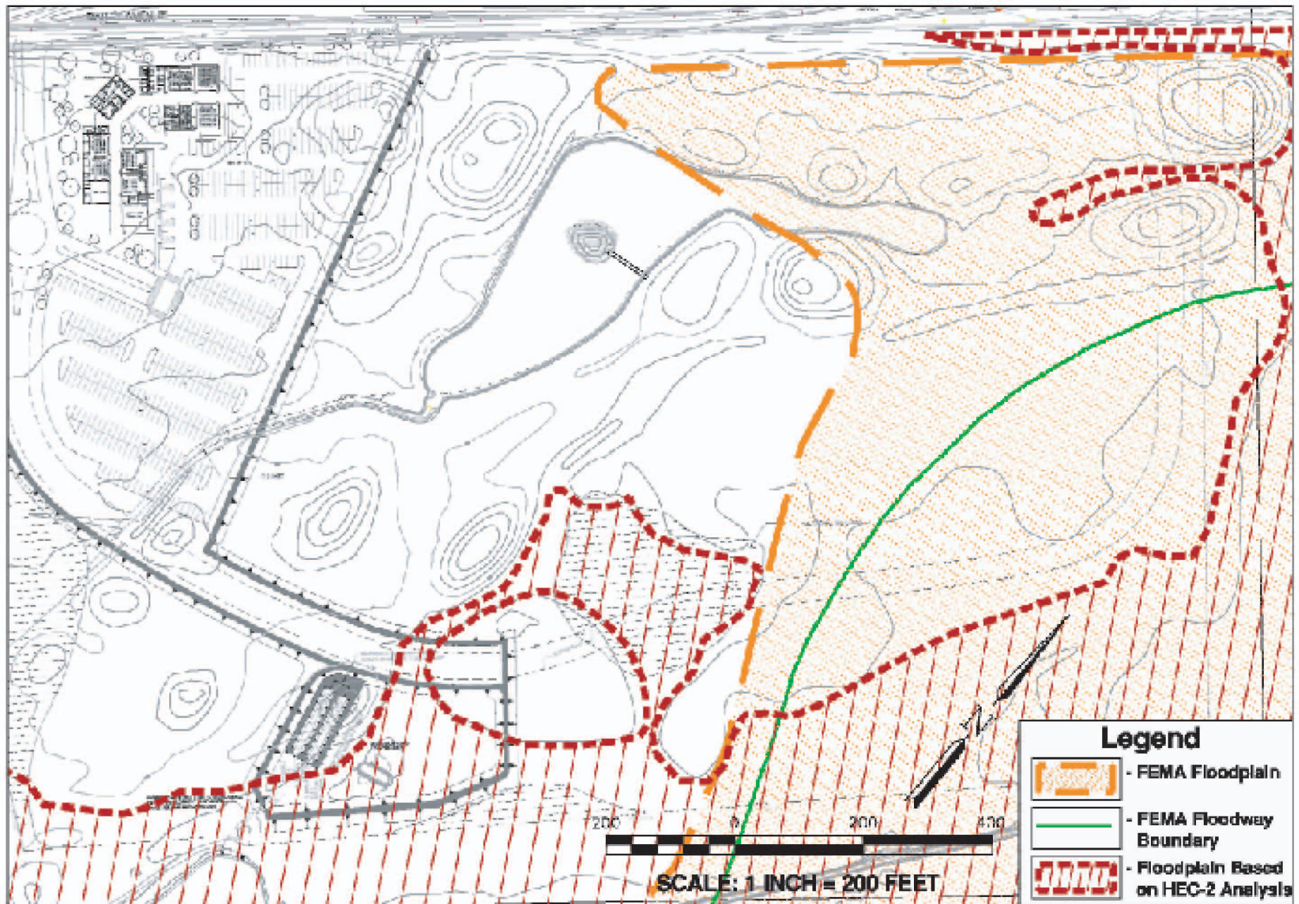
100-YEAR FLOODPLAIN WORK MAP - PHASE 1
